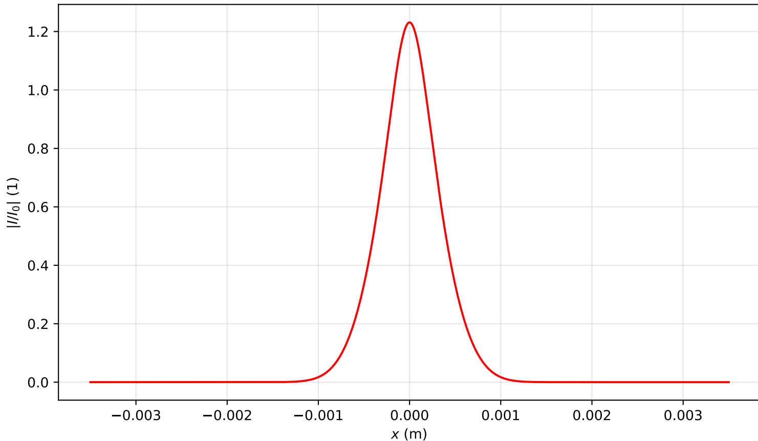
Intensity profile I(x, y = 0, z = 0.239)/I_0 , P_{in}=3.5P_{cr} , artificial time
